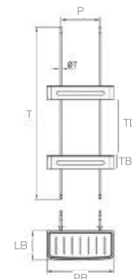
GBY7-BMK Shelf For Shower Enclosure T 72 | P 17 | TD 23.5 | PB 29 LB 12.3 | TB 5.3 cm
