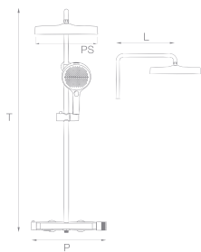
GBV88A-GM 💧 Three Function Mixer Shower Set
